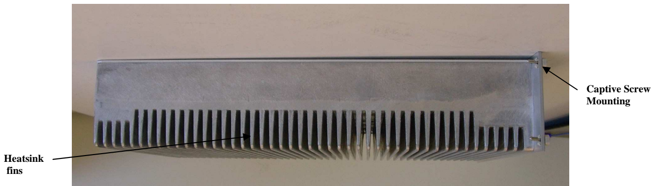
Figure 3 HePA1900 V3 side view
