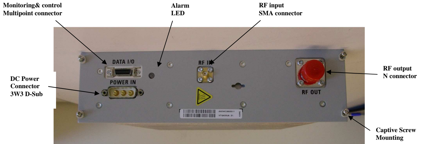
Figure 2 HePA1900 V3 Face plate view
