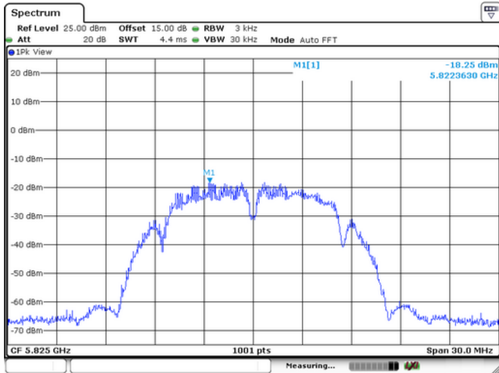
Power Density Plot on Configuration IEEE 802.11a/5825MHz
