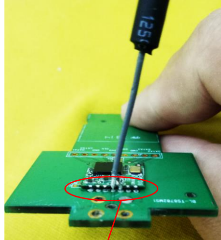
Connection Board – Back photo
