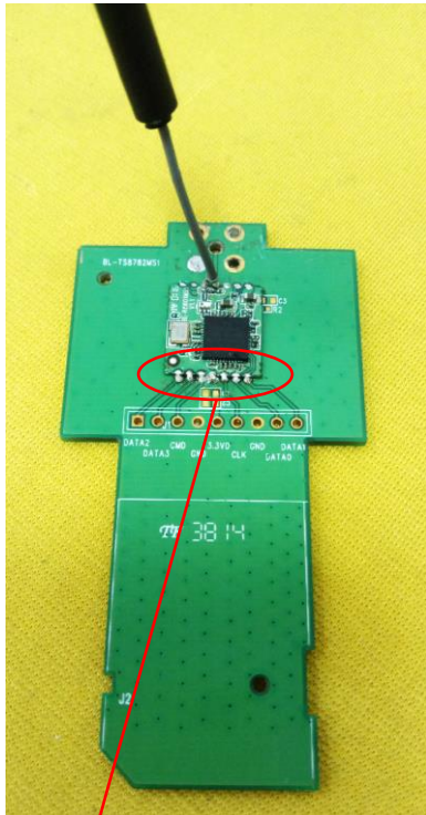
Connection Board – Front photo
