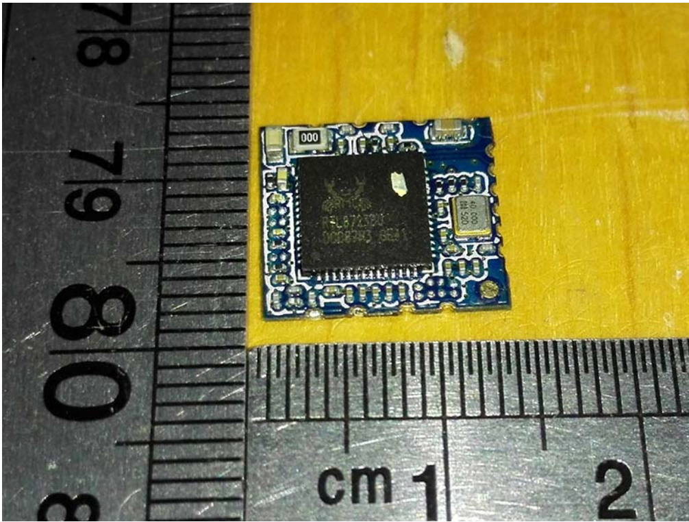
Photos of EUT Model Name: BL-R8723BT1
