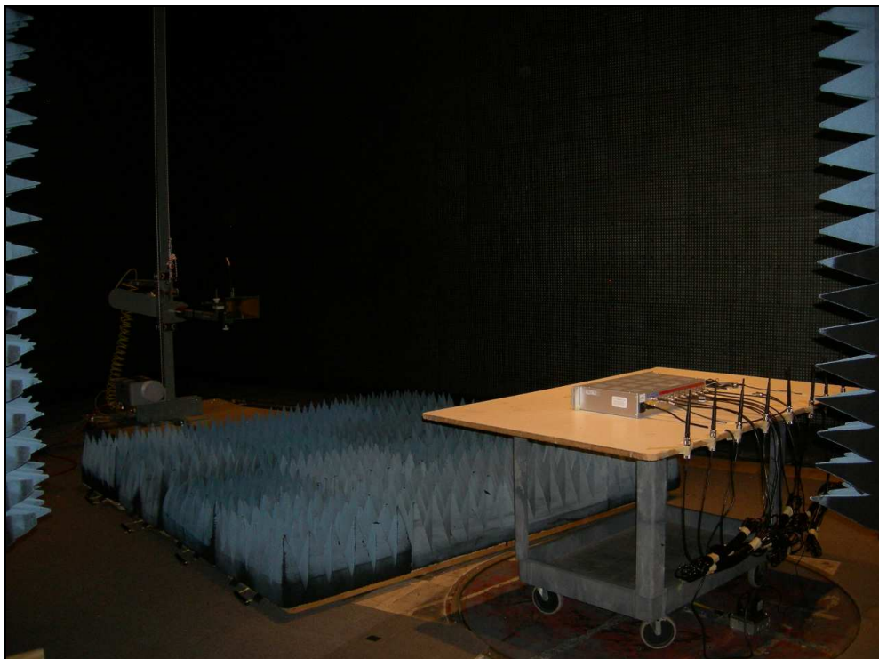
Figure 6: Radiated Emissions – Whip Antenna ZPOS
