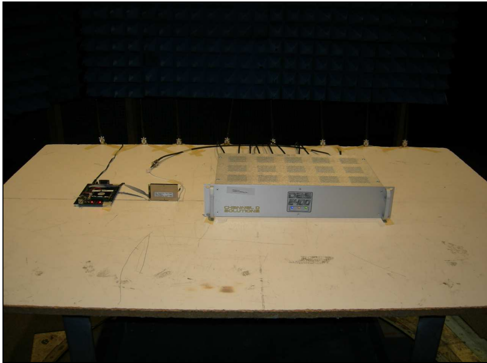
Figure 5: Radiated Emissions – Whip Antenna ZPOS
