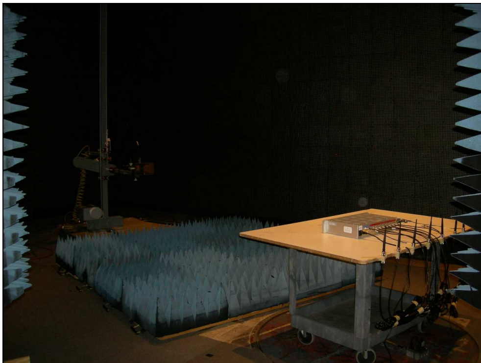
Figure 2: Radiated Emissions – Whip Antenna XPOS
