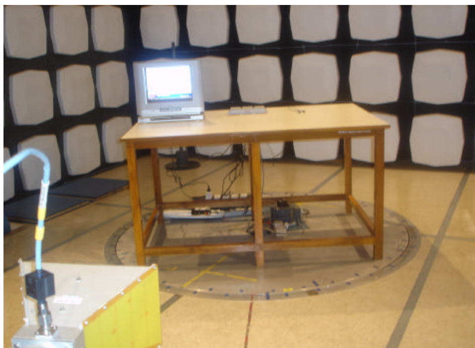
Photograph 3: Set-up for Radiated Emission in Horizontal Orientation
