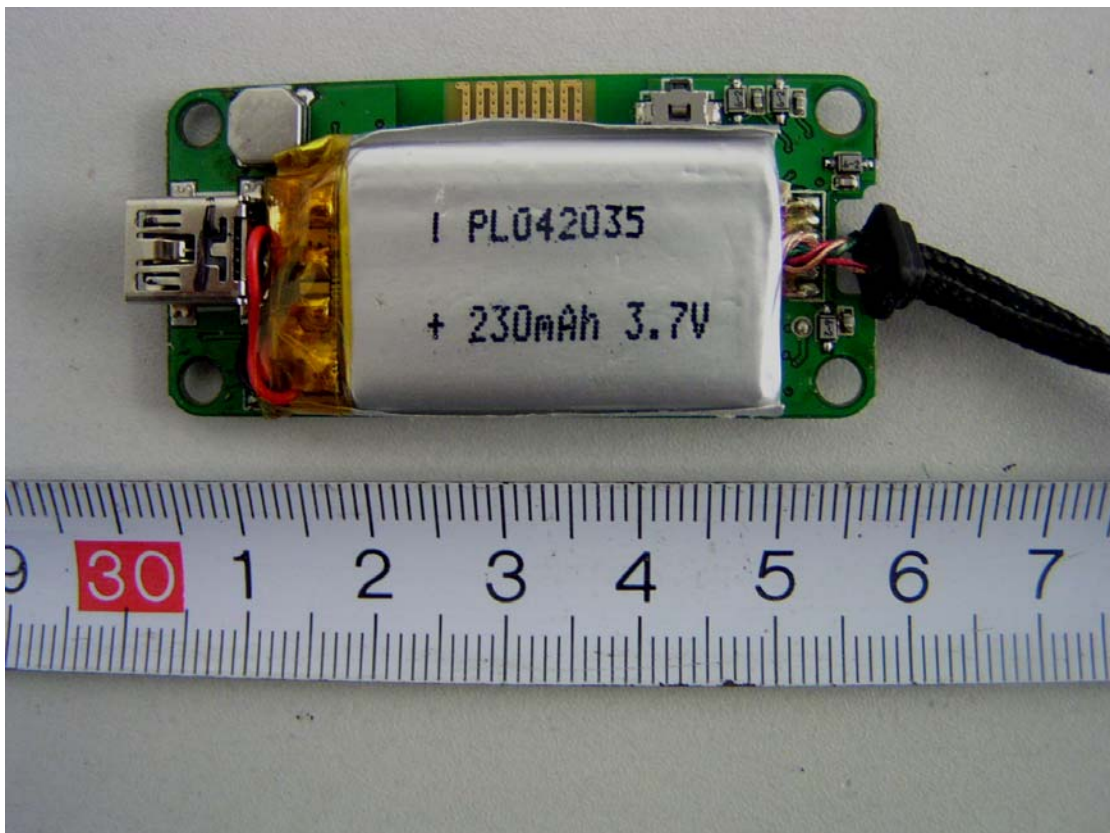
EUT – Main Board and Battery View
