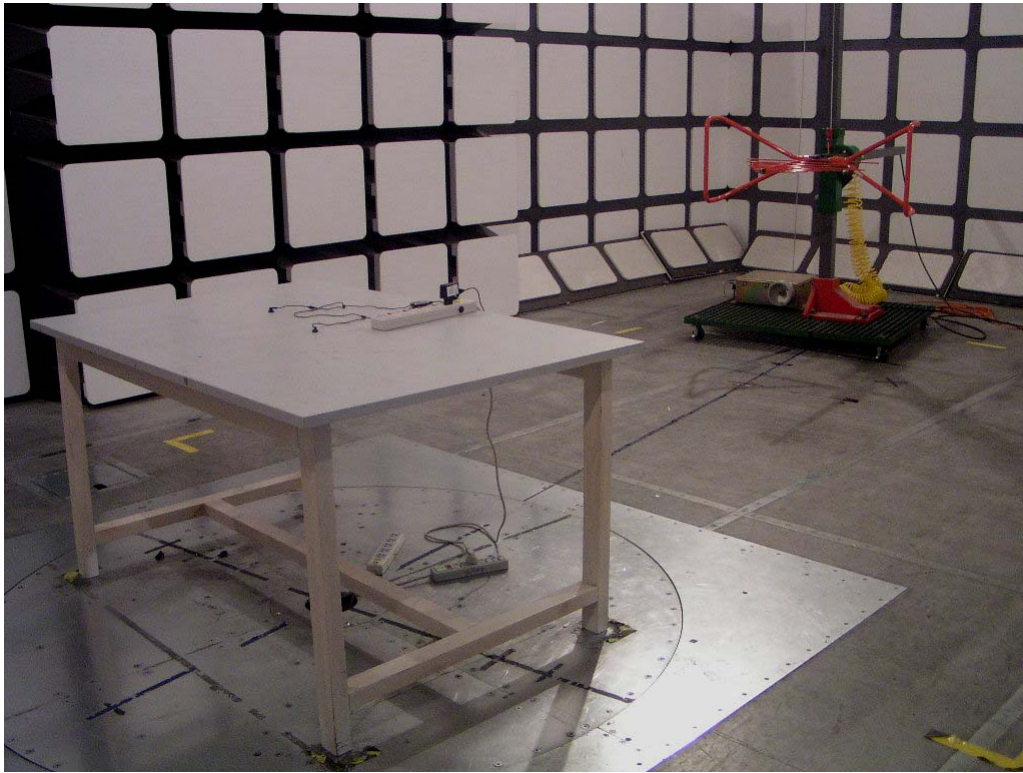
Radiated Emissions - Rear View for charging mode
