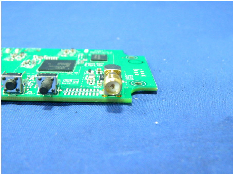
Reverse Polarity SMA connector
