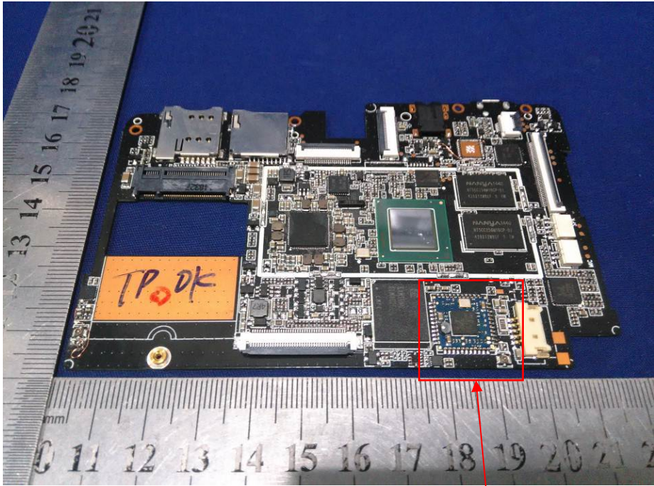
Wifi/Bluetooth Module
