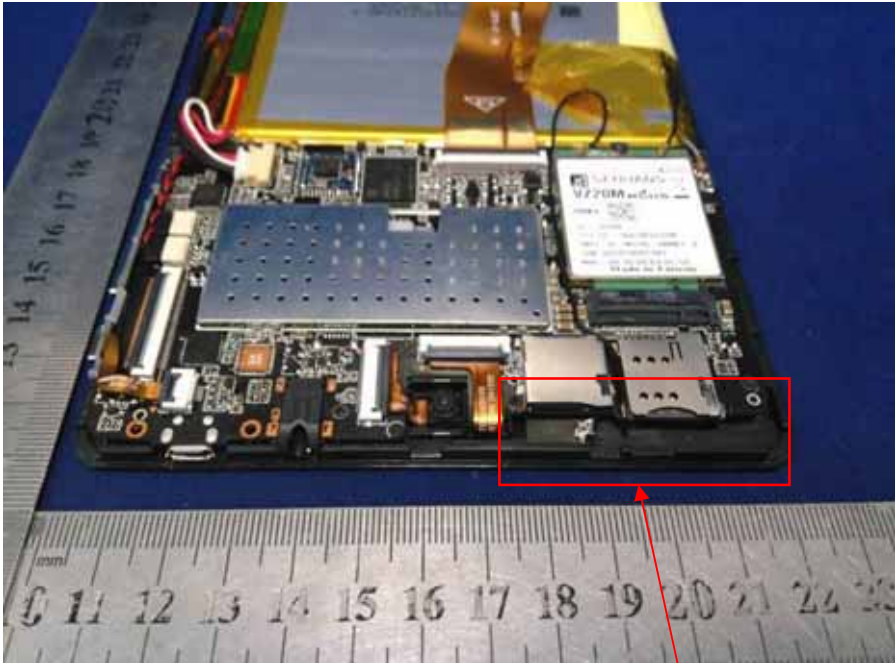
4G Antenna/Auxiliary Antenna(RX Only)
