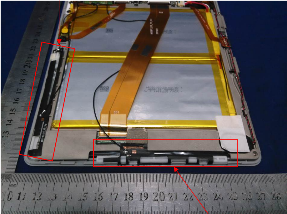
4G Antenna/Auxiliary Antenna
