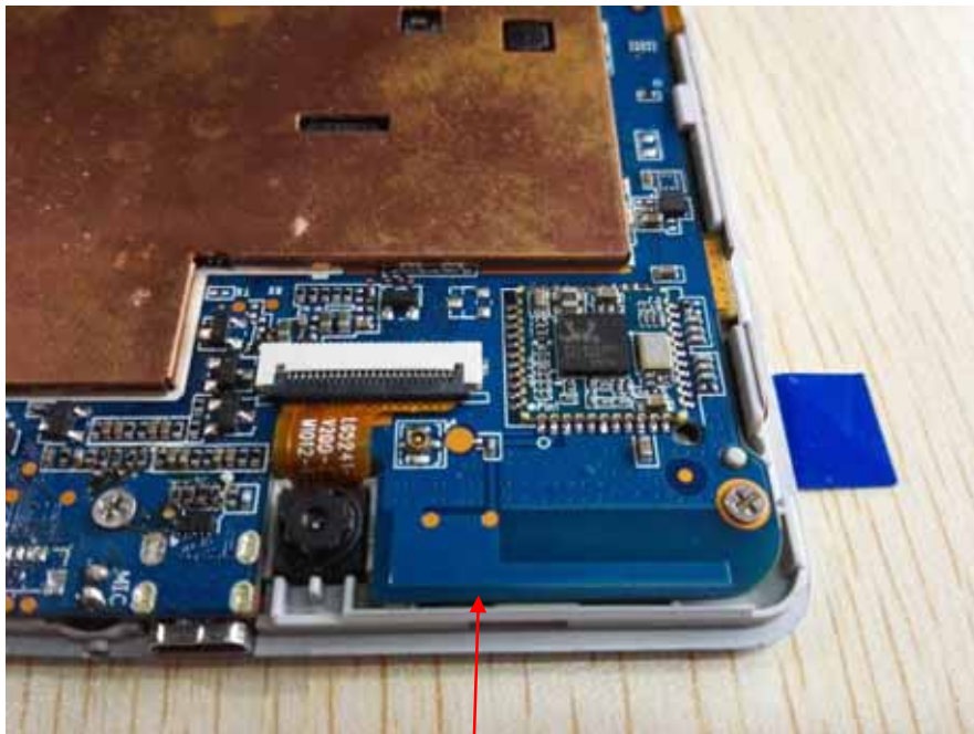
WiFi+BT Antenna
