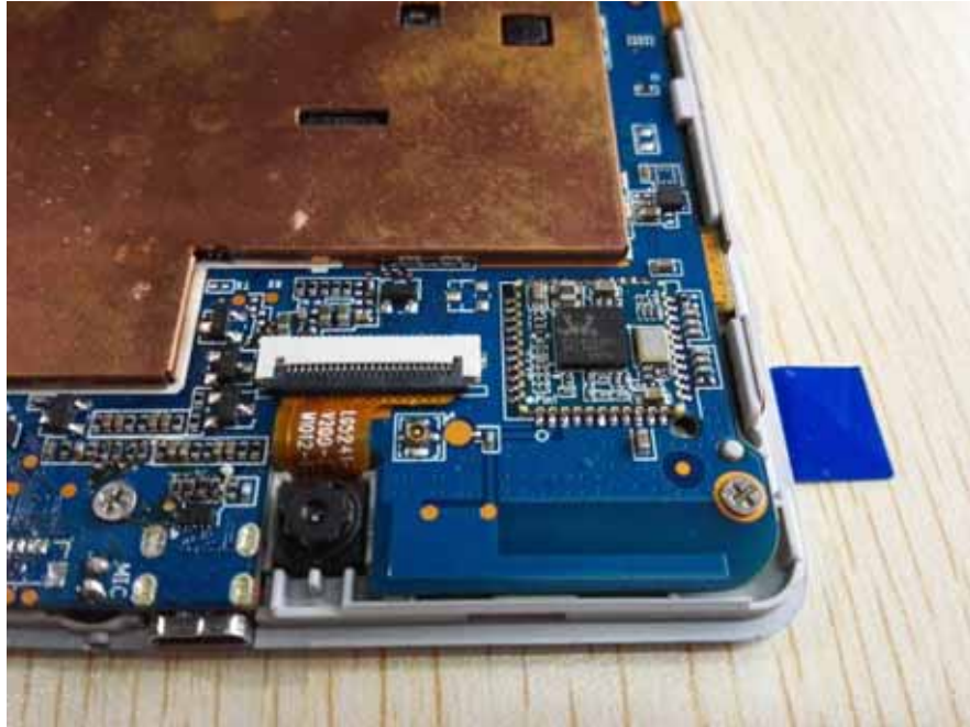
WIFI+BT Antenna
