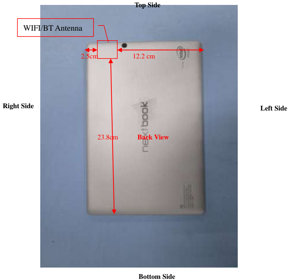
Block Diagram for EUT Antenna Position
