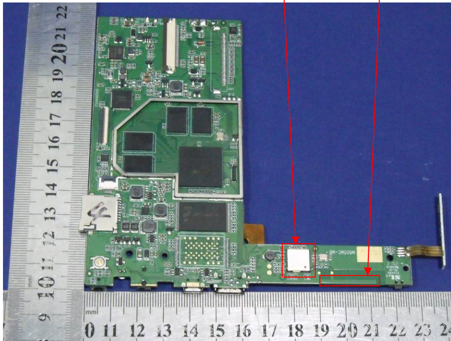
WIFI Module WIFI Antenna
