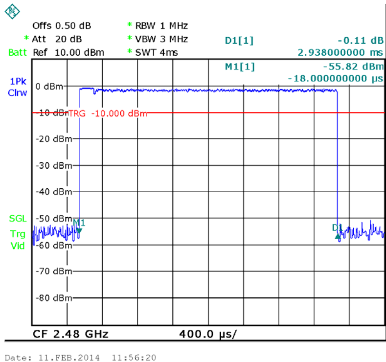
Data Packet: DH5, High channel
