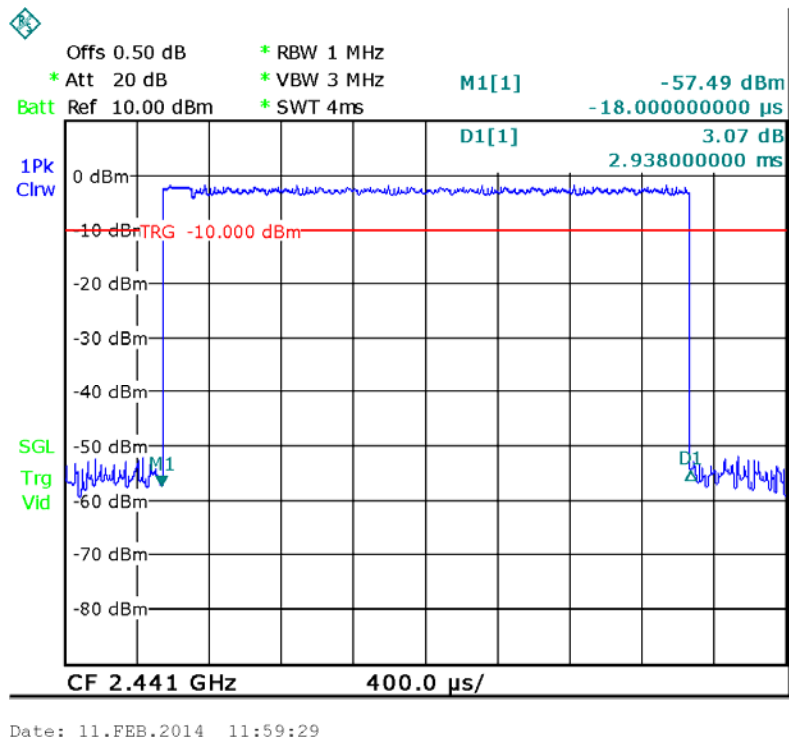
Data Packet: DH5, Middle channel
