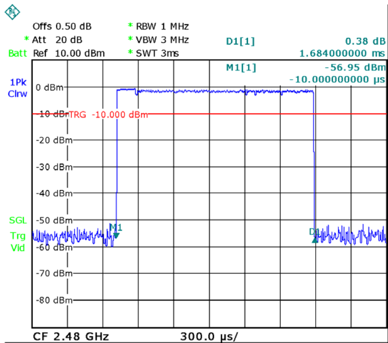
Packet:DH3, High channel
