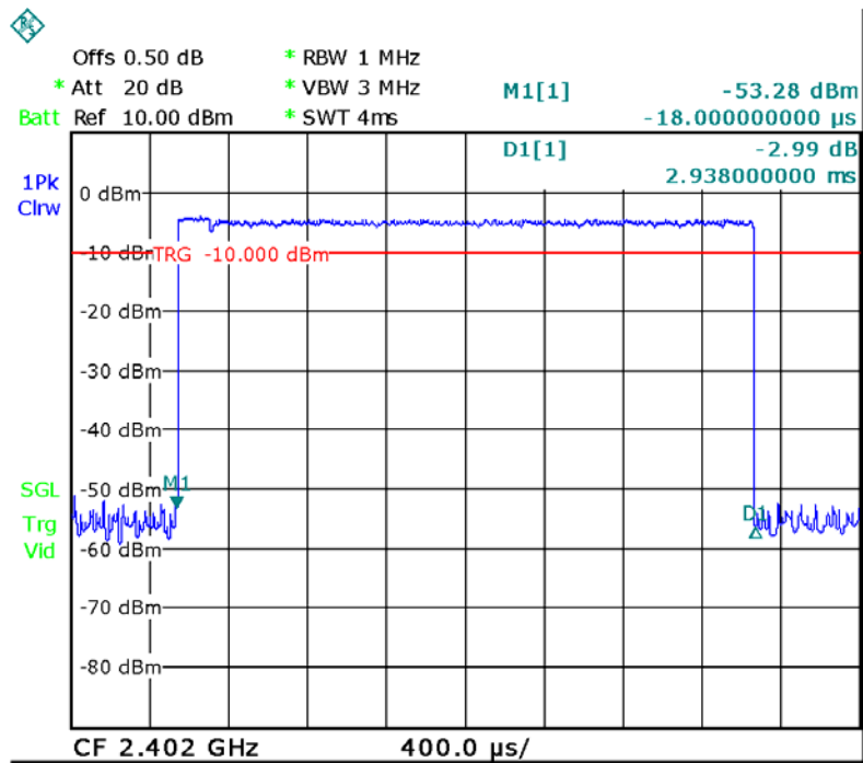
Data Packet: DH5, Low channel
