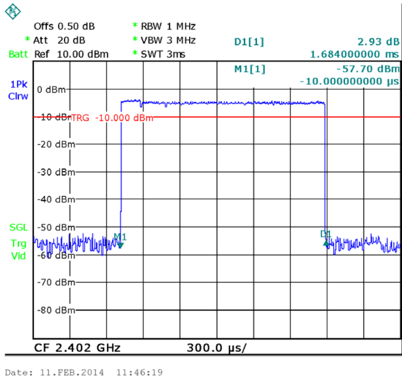
Data Packet:DH3, Low channel
