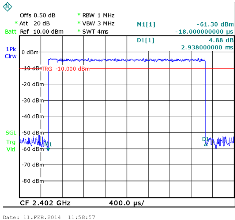
Data Packet: DH5, Low channel
