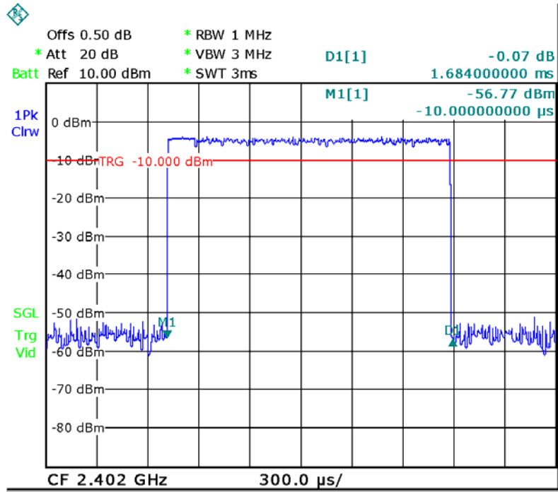
Data Packet: DH3, Low channel
