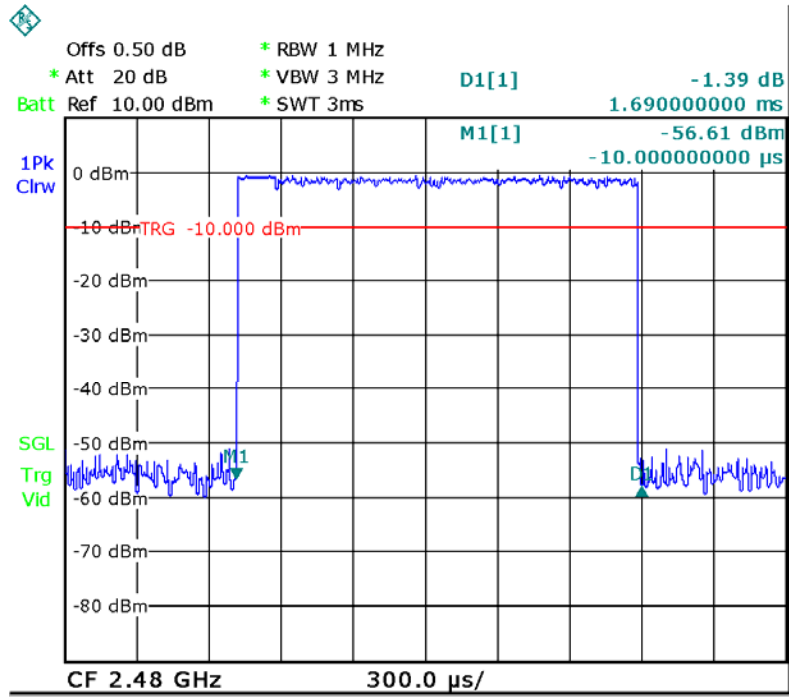
Data Packet: DH3, High channel
