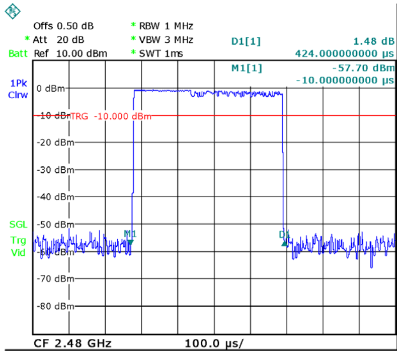
Data Packet:DH1, High channel
