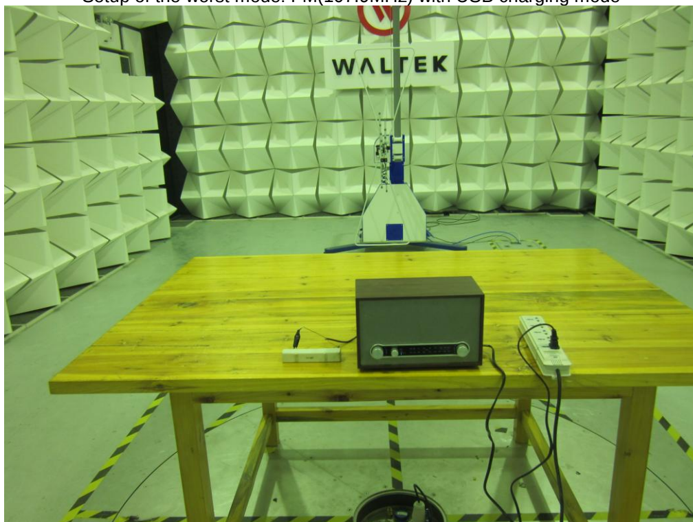
Setup of the worst mode: FM(107.9MHz) with USB charging mode
