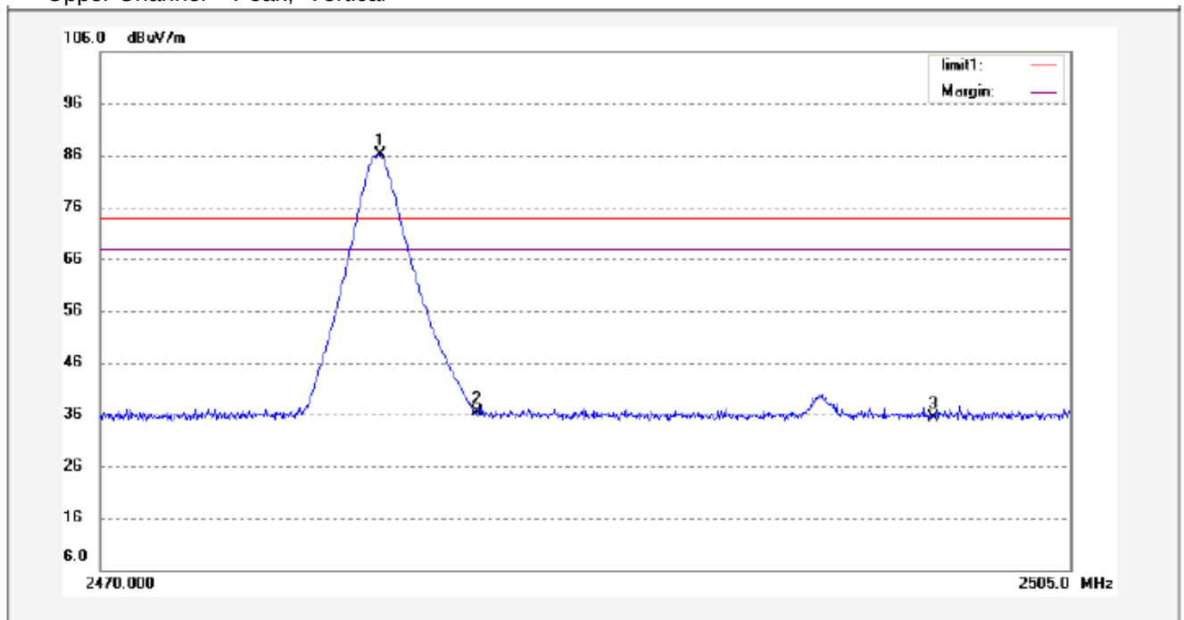
Upper Channel – Peak, Vertical
