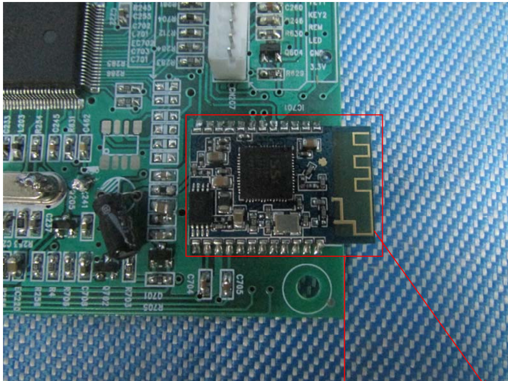
Bluetooth module PCB printed ANT.
