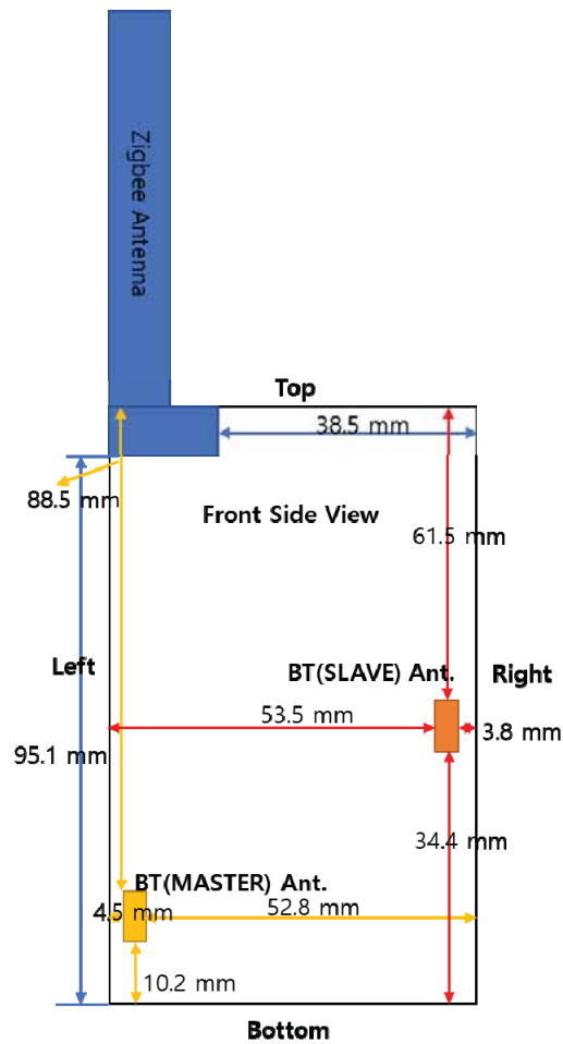
Figure F-2 Antenna Location (Zigbee Antenna Unfolded)
