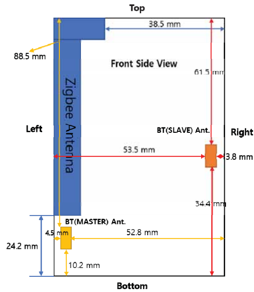
Figure F-1 Antenna Location (Zigbee Antenna Folded)
