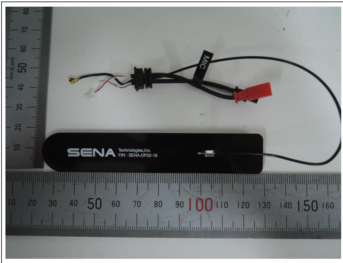
<Antenna 2(Model : SENA-DP02-19)>
