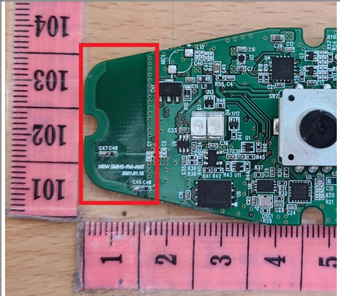
BT Antenna
