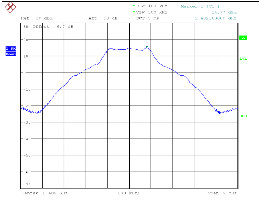
Bandedge _ Single
