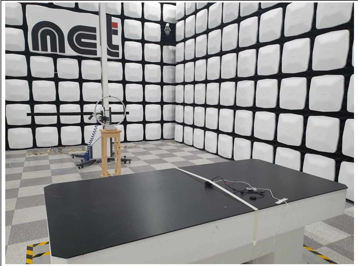
Below 30 MHz
