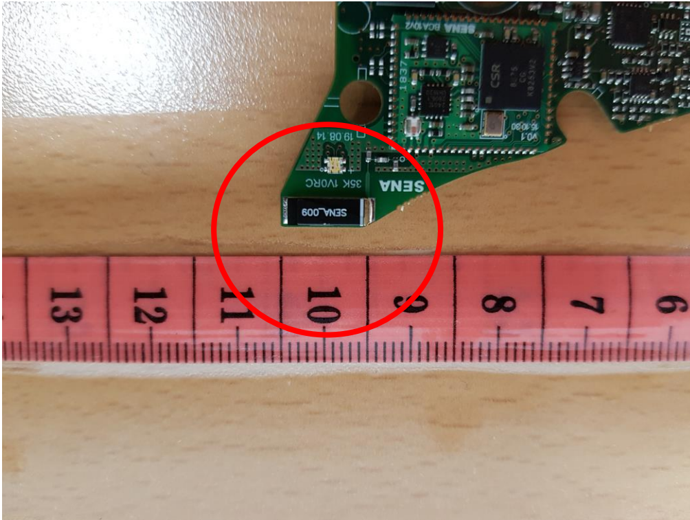
MESH Antenna
