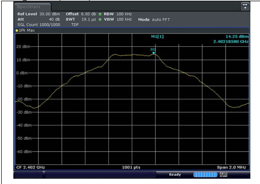
GFSK 2 402 MHz(reference)
