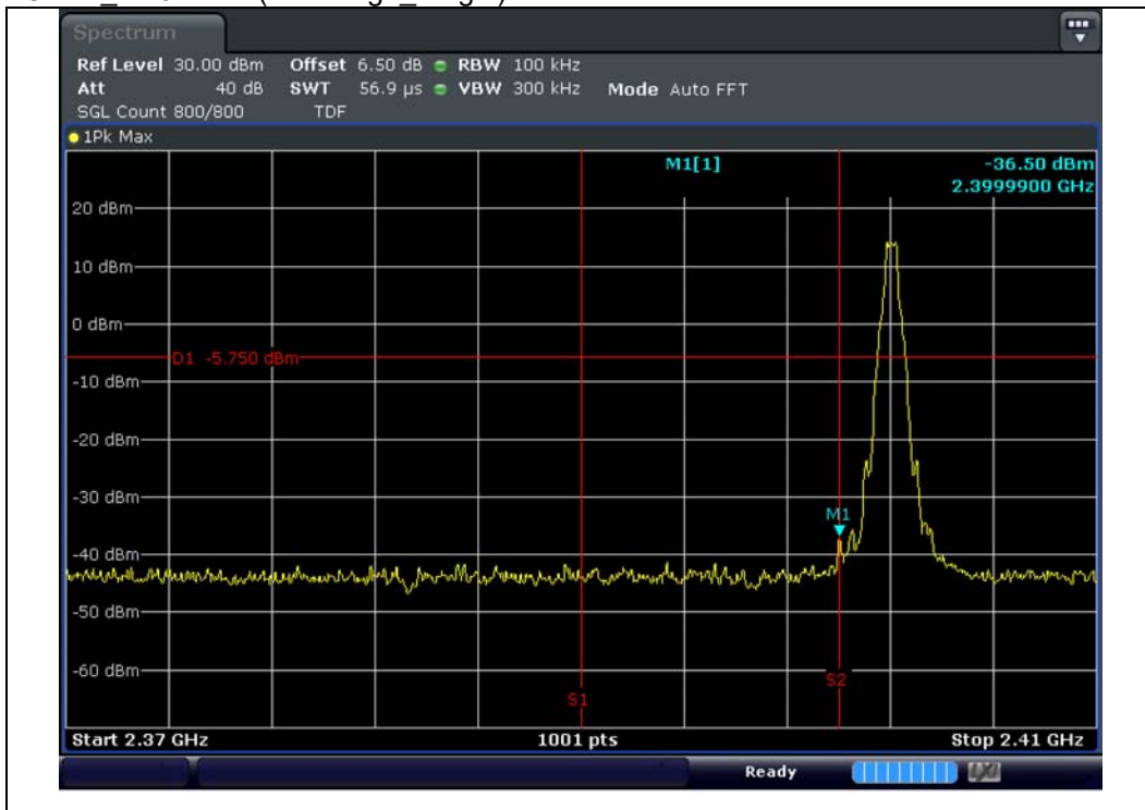
GFSK 2 402 MHz(Bandedge_Single)
