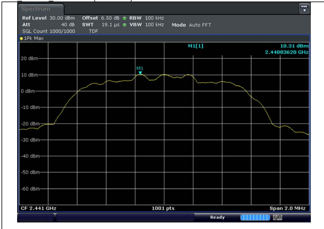
M1 8DPSK 2 441 MHz(reference)
