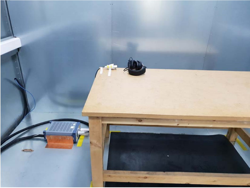
AC Conducted Power Line
