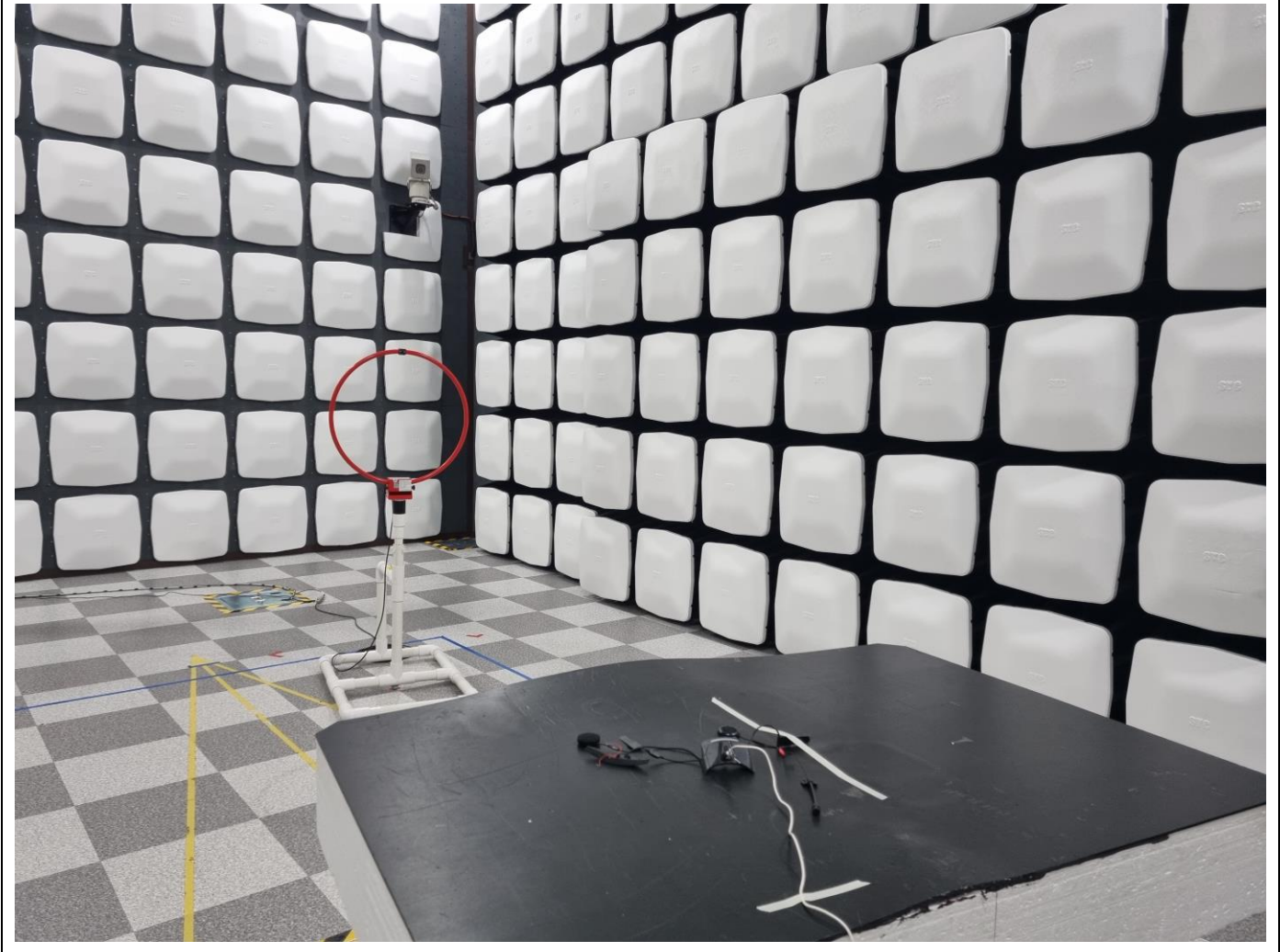
Below 30 MHz
