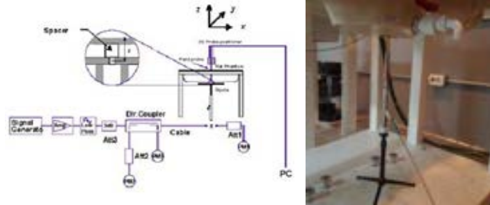
Figure 9.1 Dipole Verification kit Test Setup Diagram & Photo
