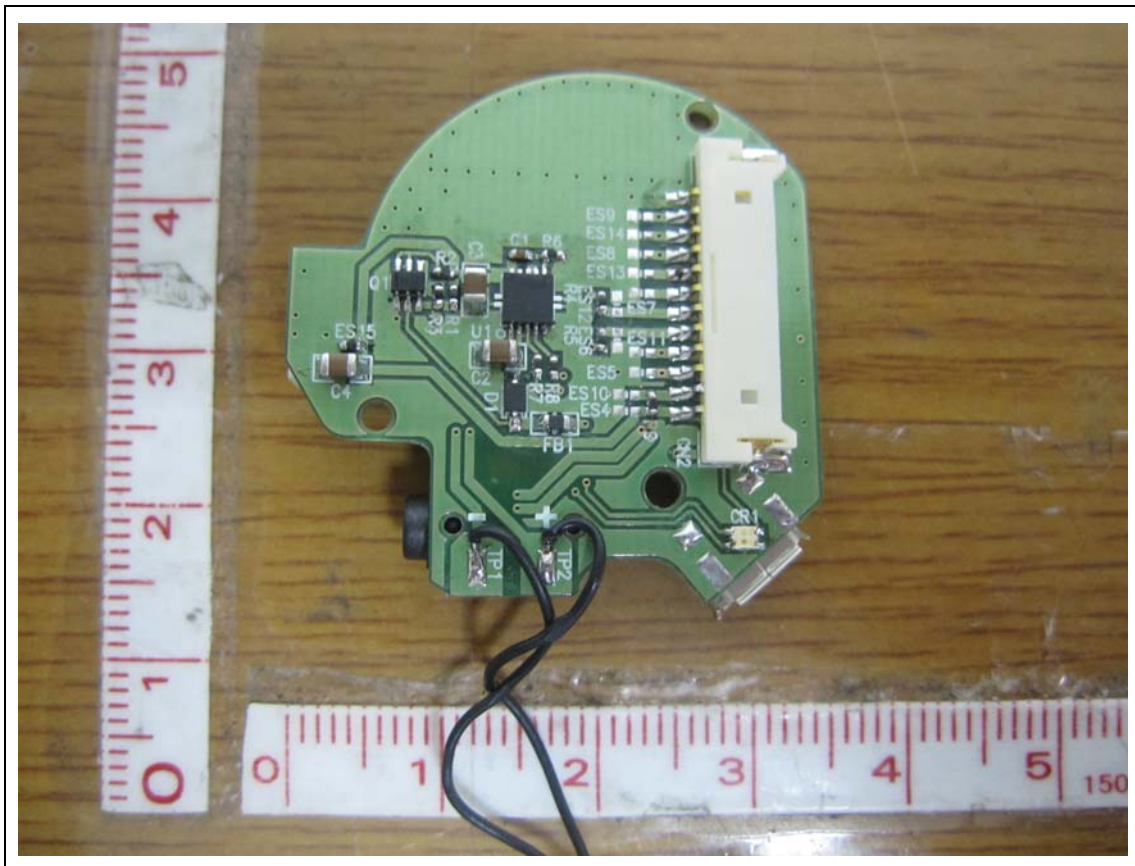
SubBoard - Rear
