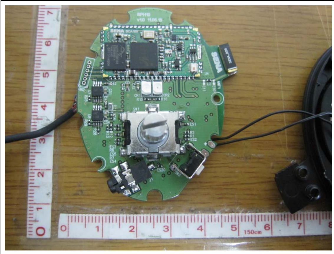
MainBoard - Rear
