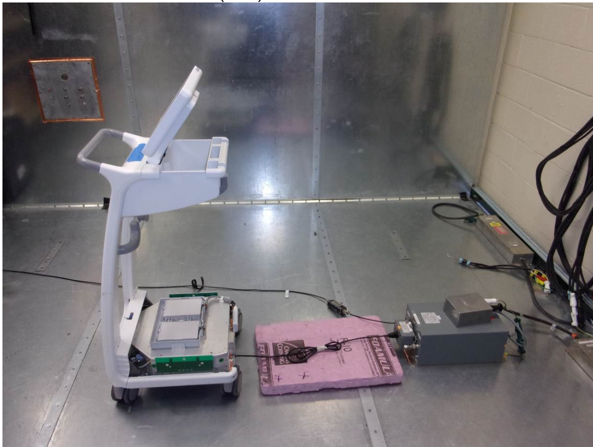
LINE CONDUCTED EMISSIONS (SIDE)
