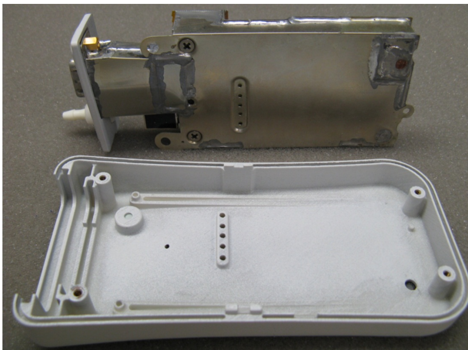
wSpO2 – Top (Removed from Enclosure)
