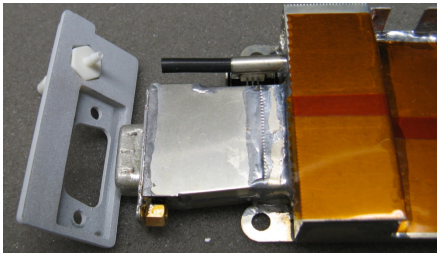
wSpO2 – Bottom (Metal Cover Removed)
