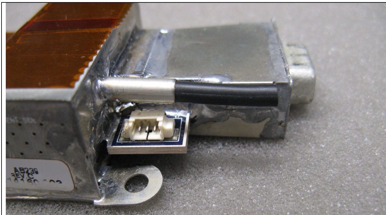
wSpO2 - Radio Board (Bottom)
