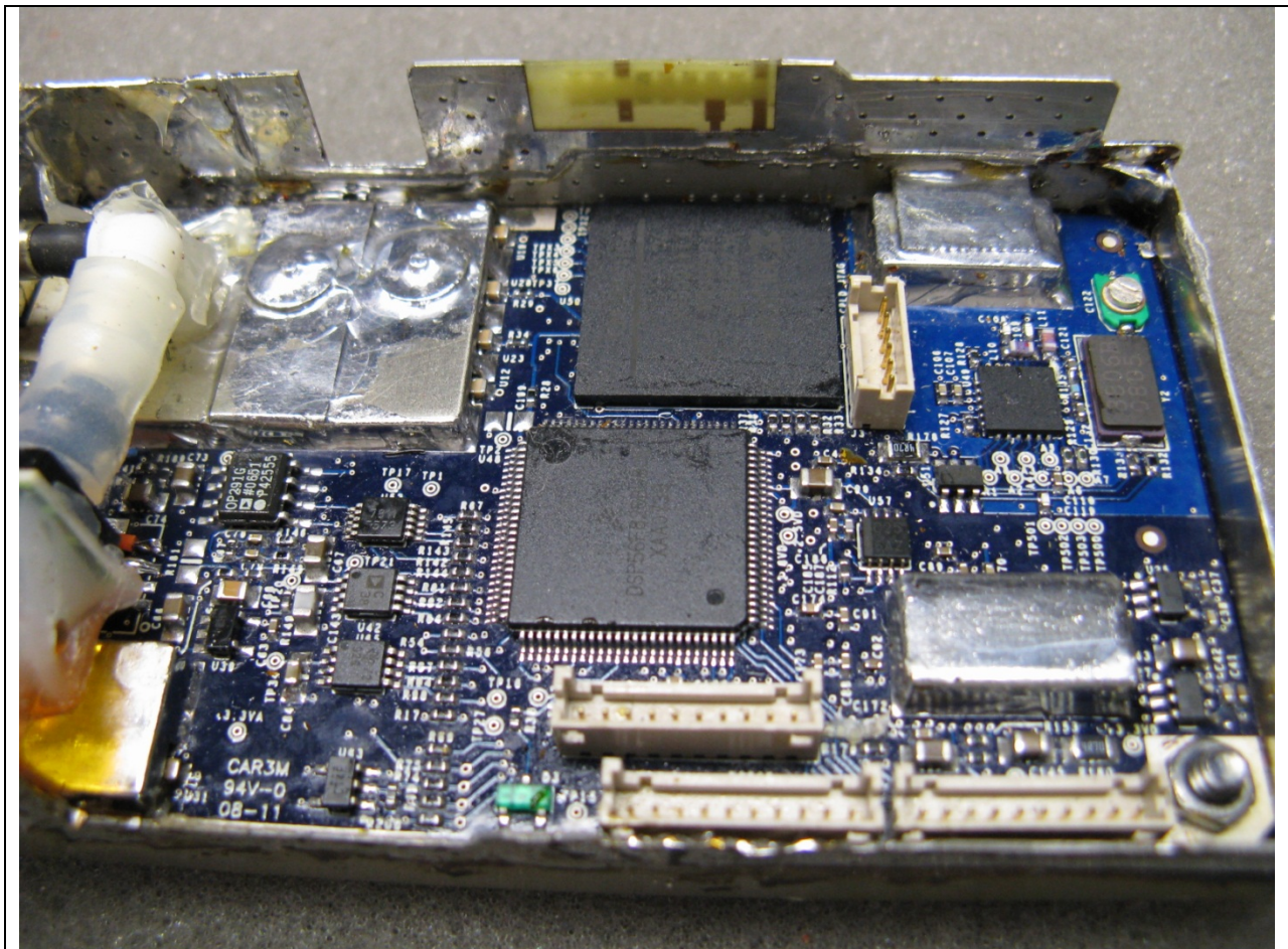
wSp02 - Top of PCB Zoomed in
