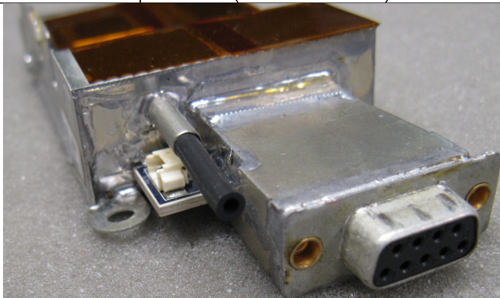
wSpO2 – Radio Circuit (Top)
