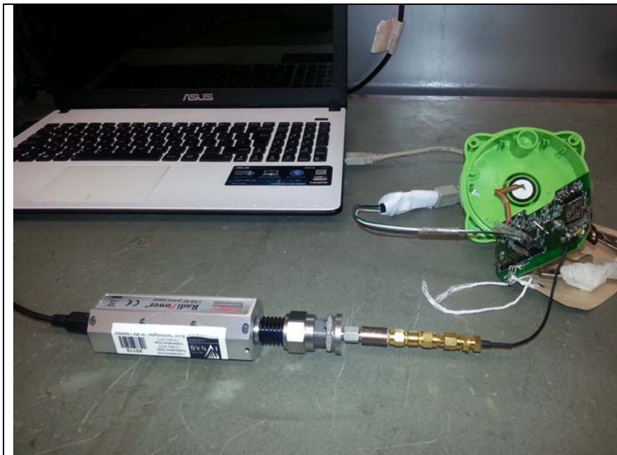
Fig 4 Test setup Conducted Emissions
