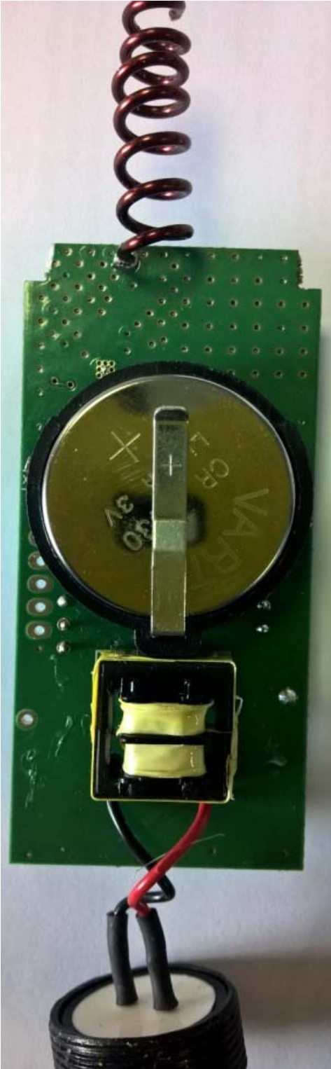
Back of PCB – with battery (lithium coin cell).
