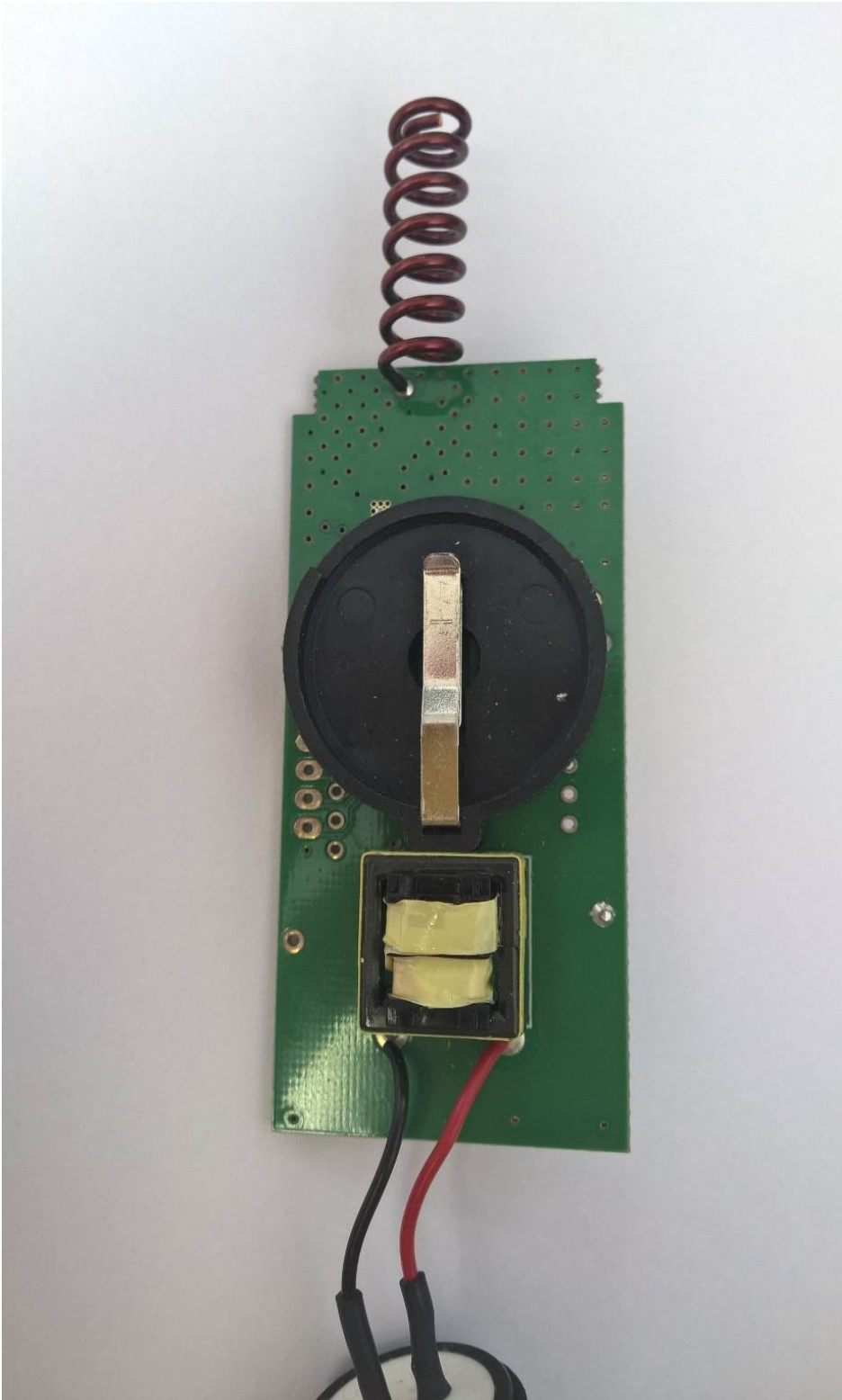
Back of PCB (Visual / Non-Visual) – Battery Removed.
