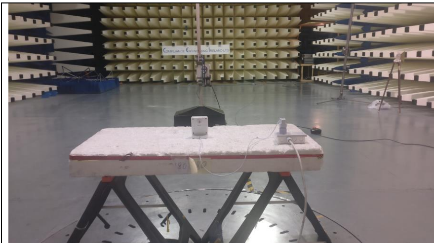
Fig 2b Test setup 300MHz -1GHz Rad Emissions
