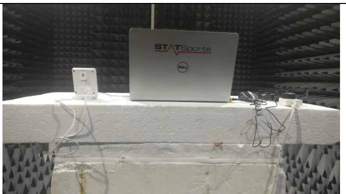
Fig C6 Radiated Emissions
