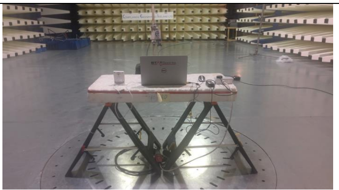
Fig C4 Radiated Emissions
