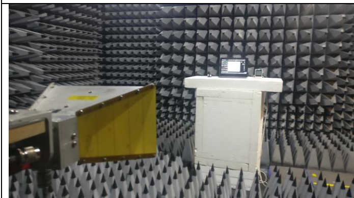
Fig C5 Radiated Emissions
