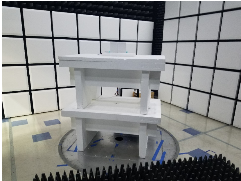
19deg and 25deg Units Radiated Spurious Emissions
