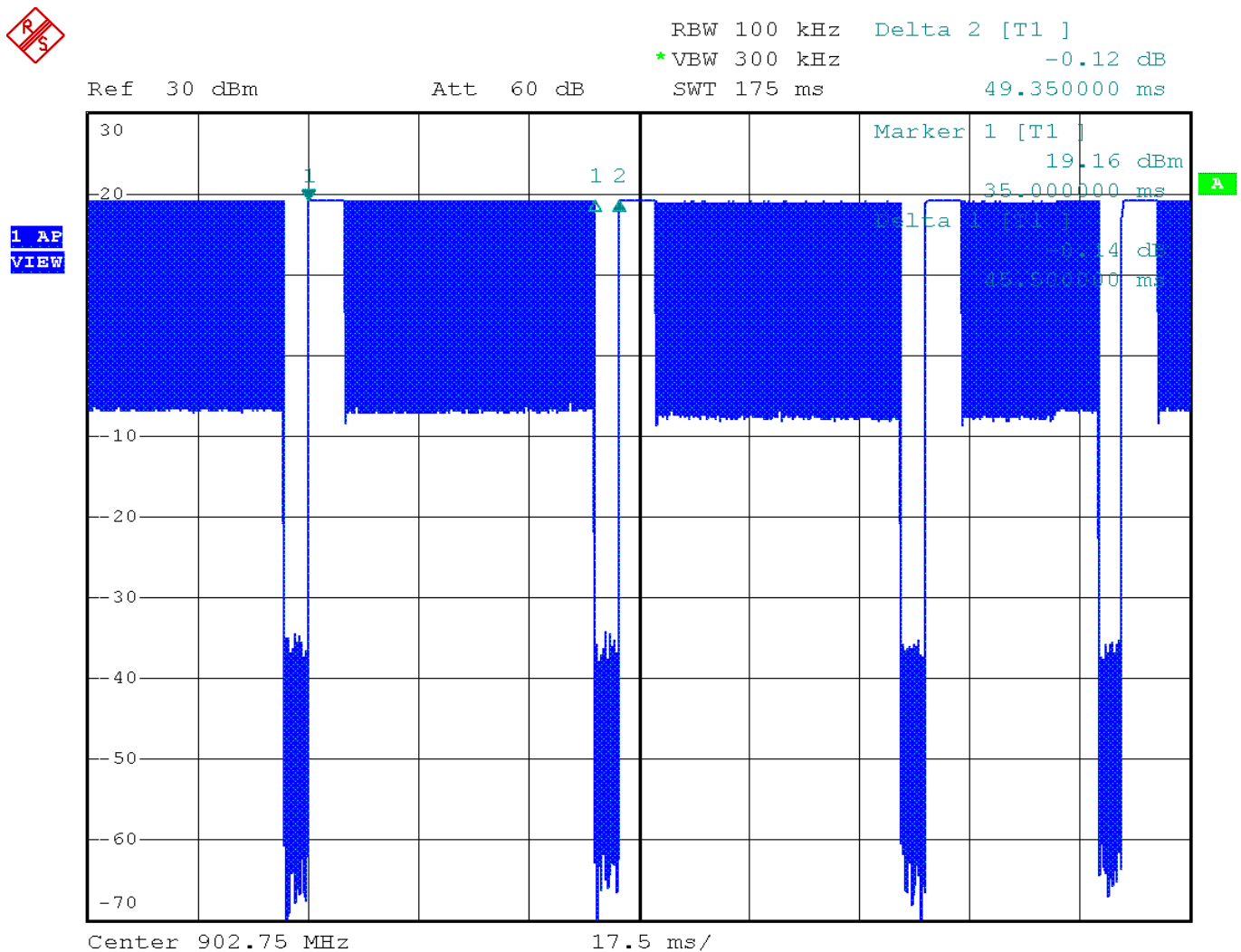
Time-domain plot for UHF RFID transmission signal
