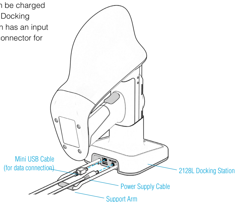
Figure 2: Charging the 2128L UHF Reader
