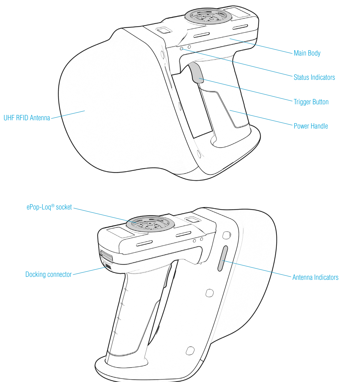
Figure 1: 2128L Reader with UHF RFID Antenna, 2D Laser Barcode Imager and Power Handle
