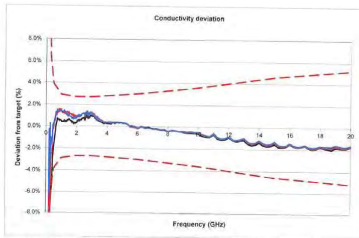
Fig. 3.2 Methanol conductivity deviation from target, 200 MHz – 20 GHz
