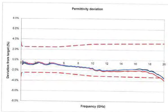
Fig. 4.1 HSL permittivity deviation from target, 200 MHz – 20 GHz
