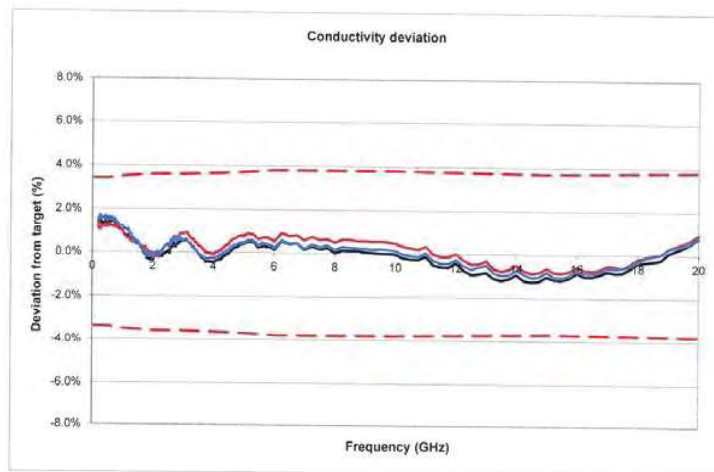
Fig. 4.2 HSL conductivity deviation from target, 200 MHz – 20 GHz
