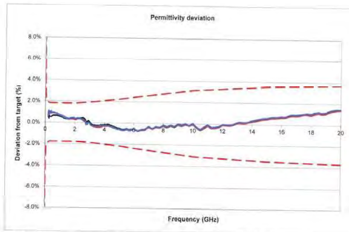
Fig. 3.1 Methanol permittivity deviation from target, 200 MHz – 20 GHz
