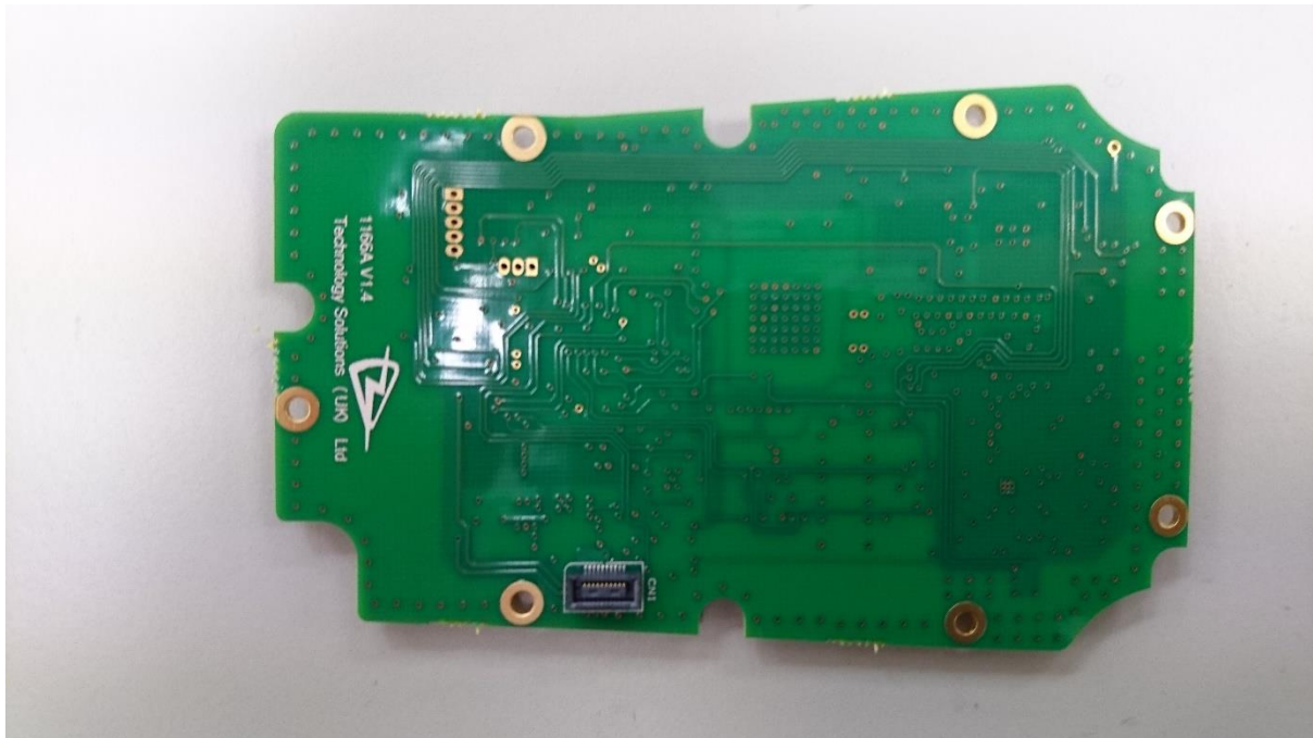
RFID board (1166A TSL01967) rear view
