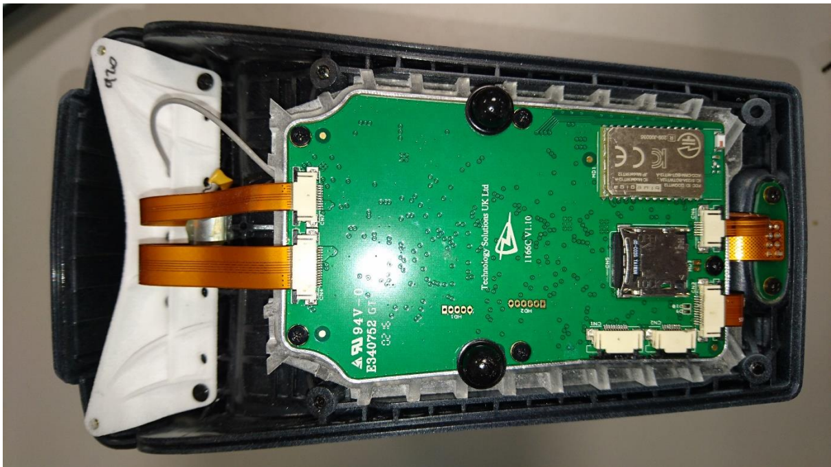
View into top of reader with cover removed
