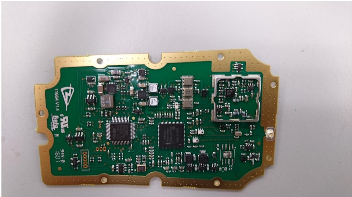
RFID board (1166A TSL01967) top view (PA screening can removed)
