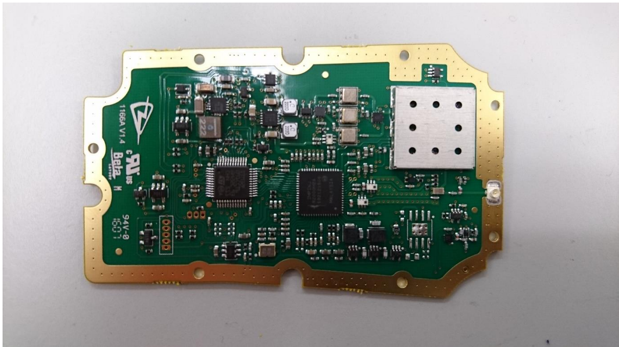
RFID board (1166A TSL01967) top view (PA screening can fitted)
