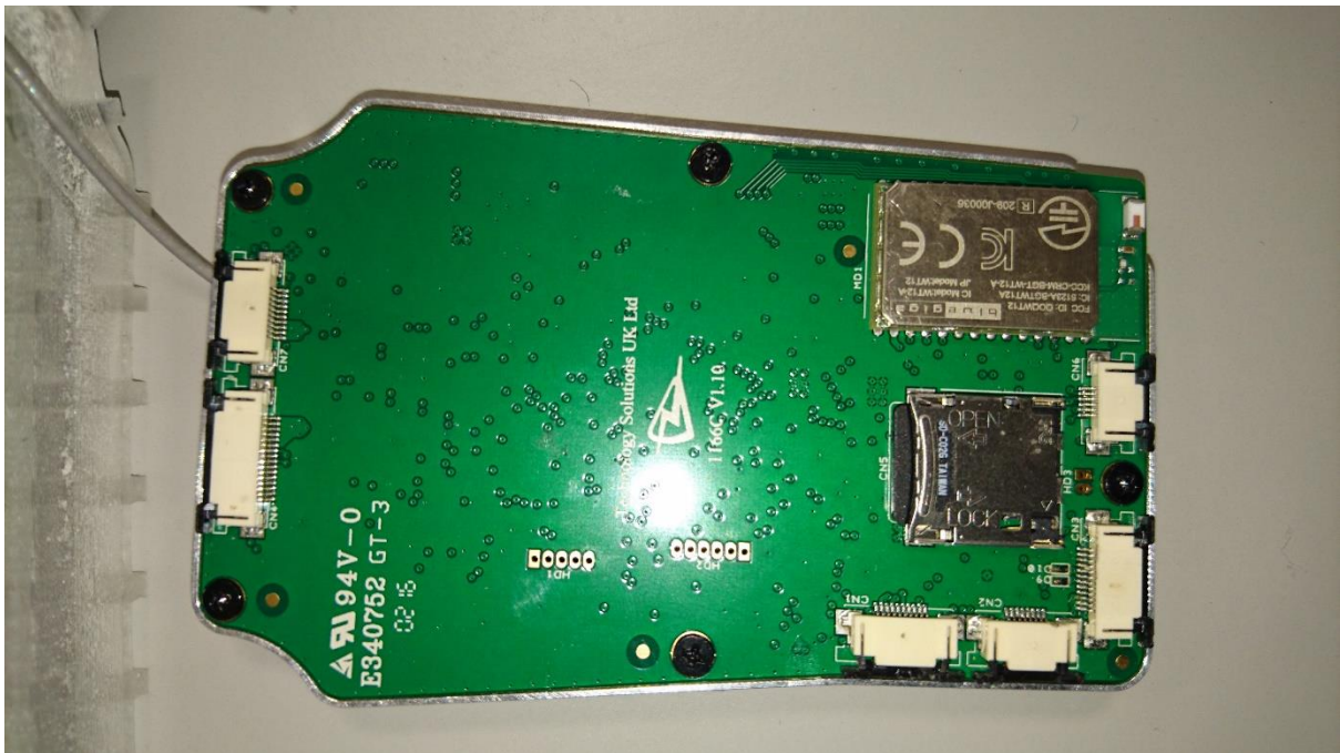
Electronic assembly top view / control board rear view
