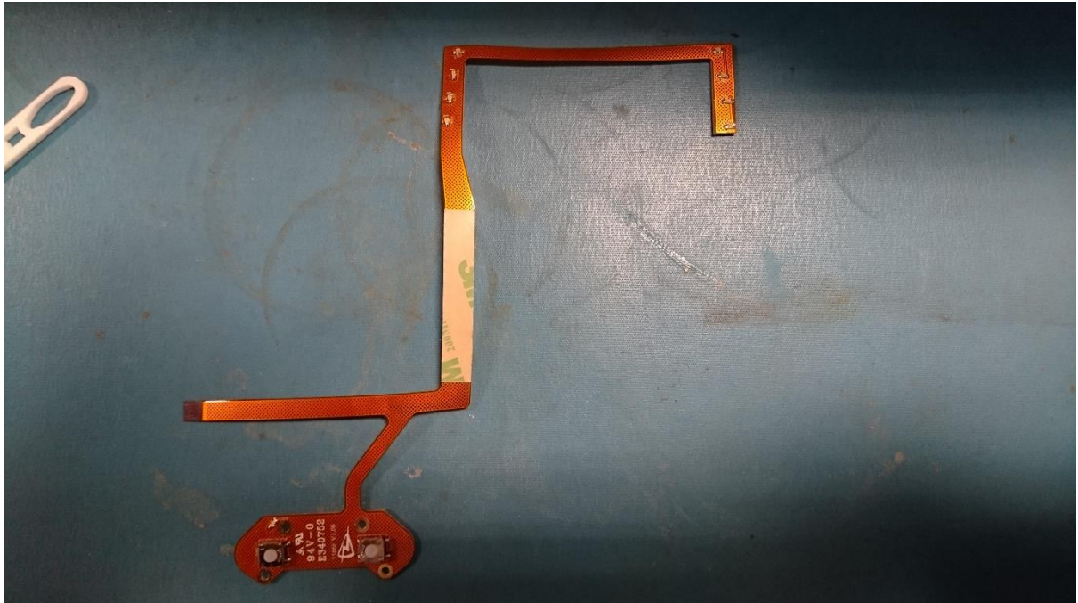
Status LED and Rear Buttons flexible circuit 1166F TSL01950
