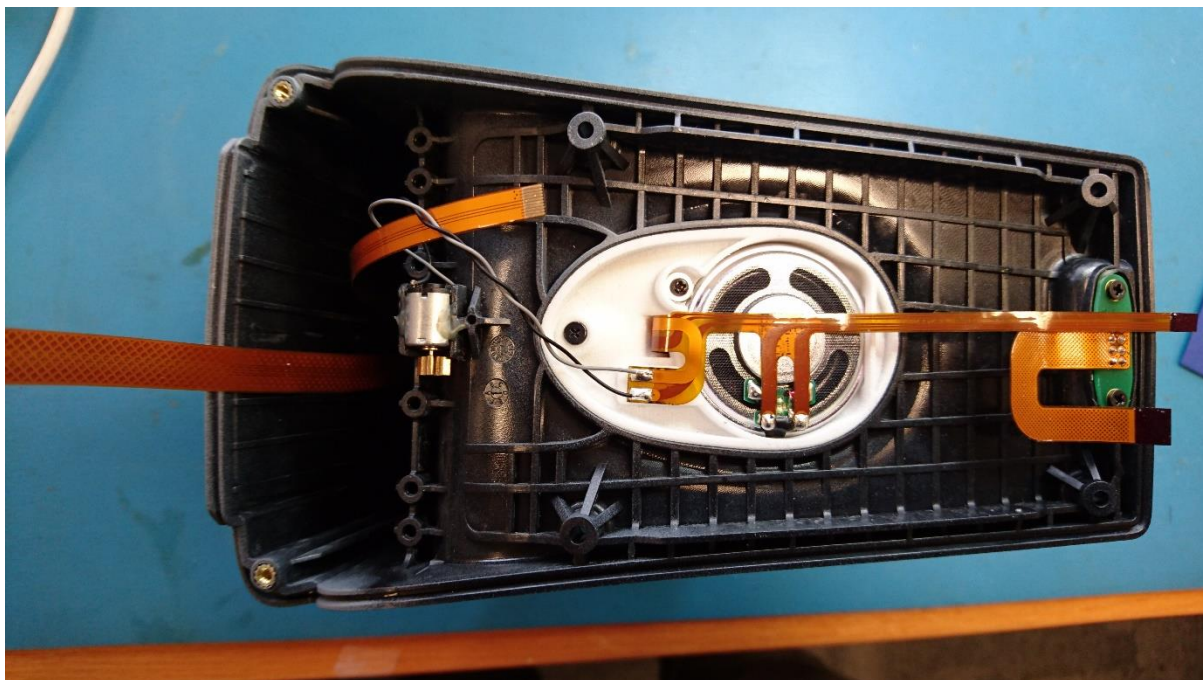
View into reader with electronic assembly removed
