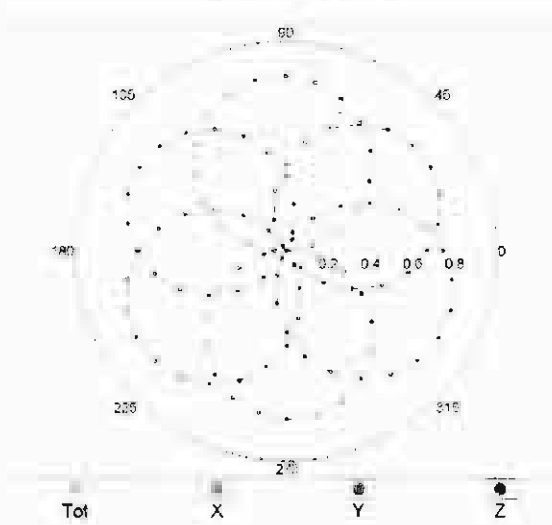
f=600 MHz,TEM
