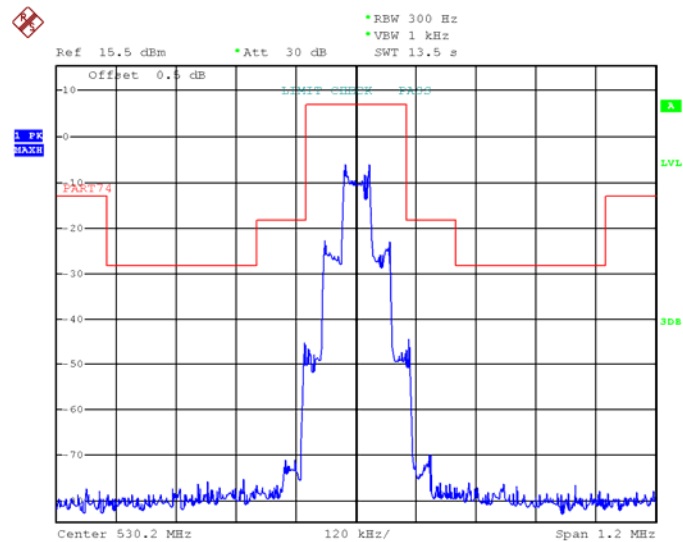
Emission Mask
