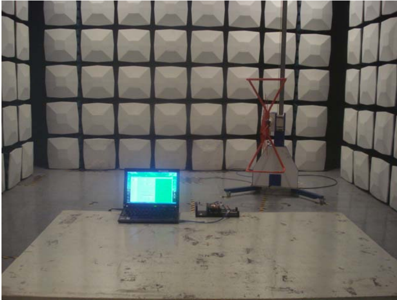
Radiated Emissions View (Below 1GHz)
