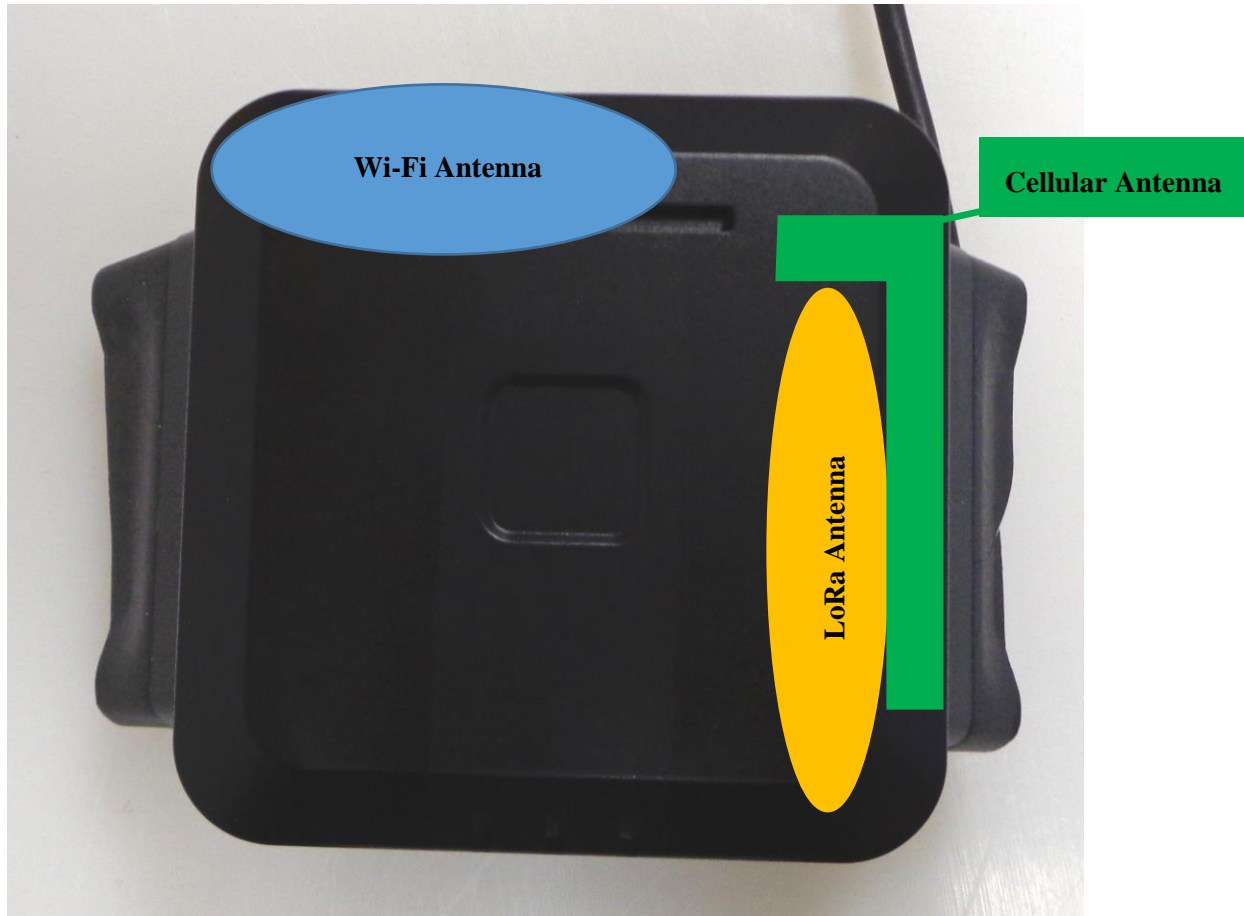
Photo 1: Antenna Locations (Front View)
