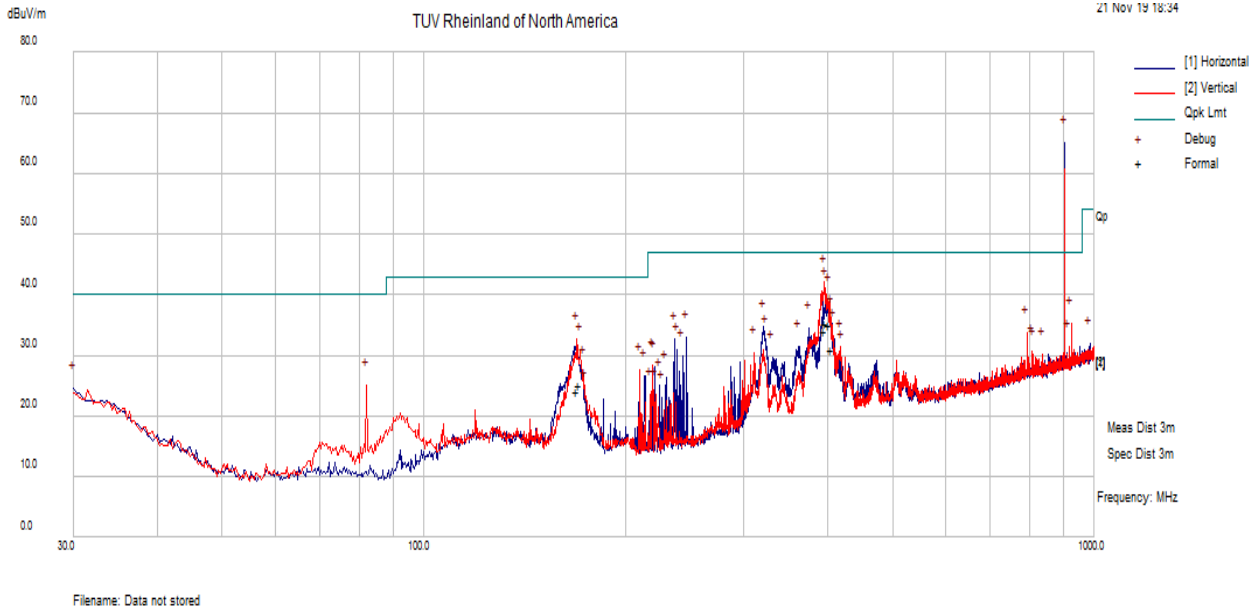
Radiated Emissions 30-1000 MHz.
