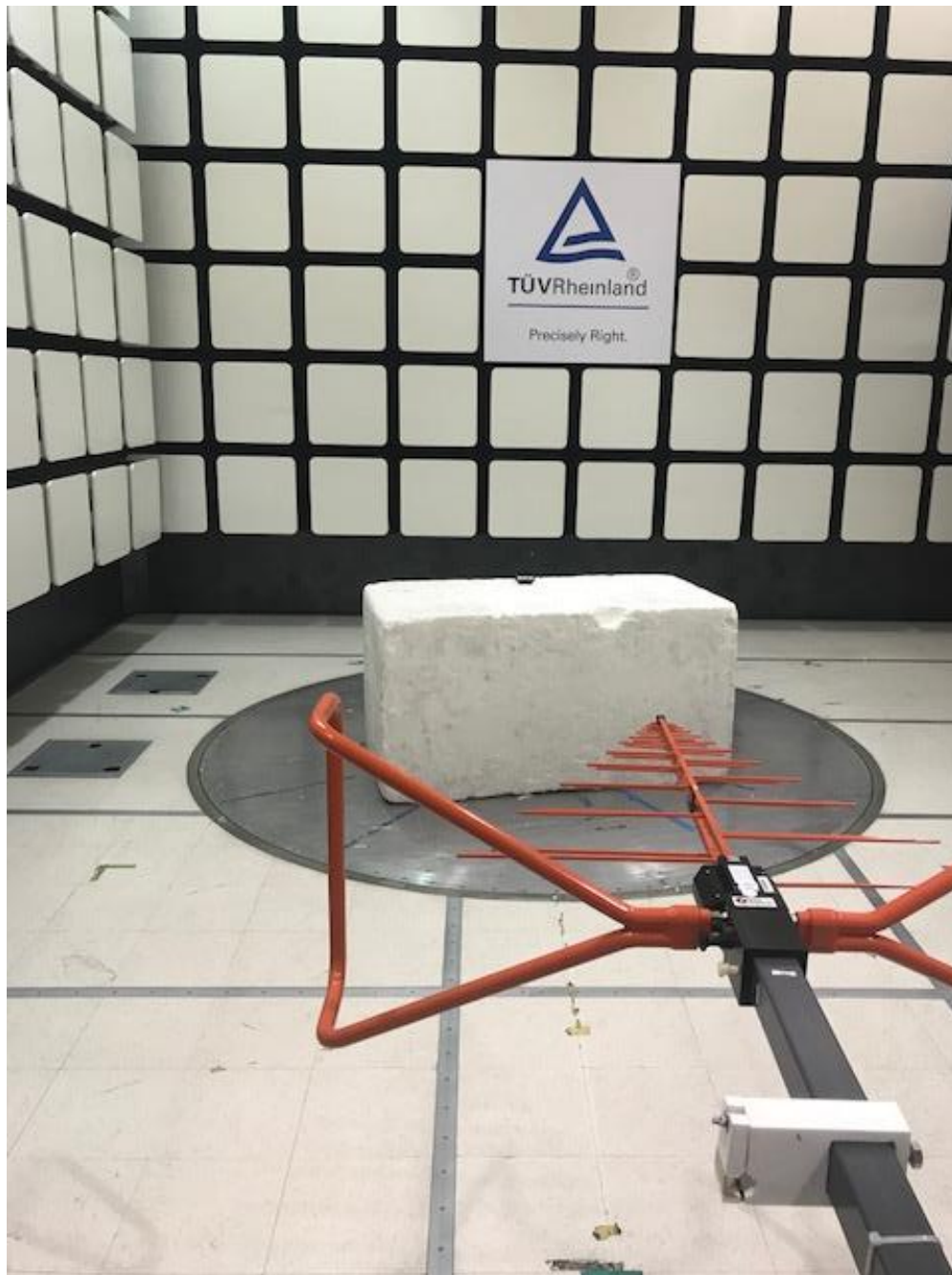
Test Setup 30-1000 MHz Front
