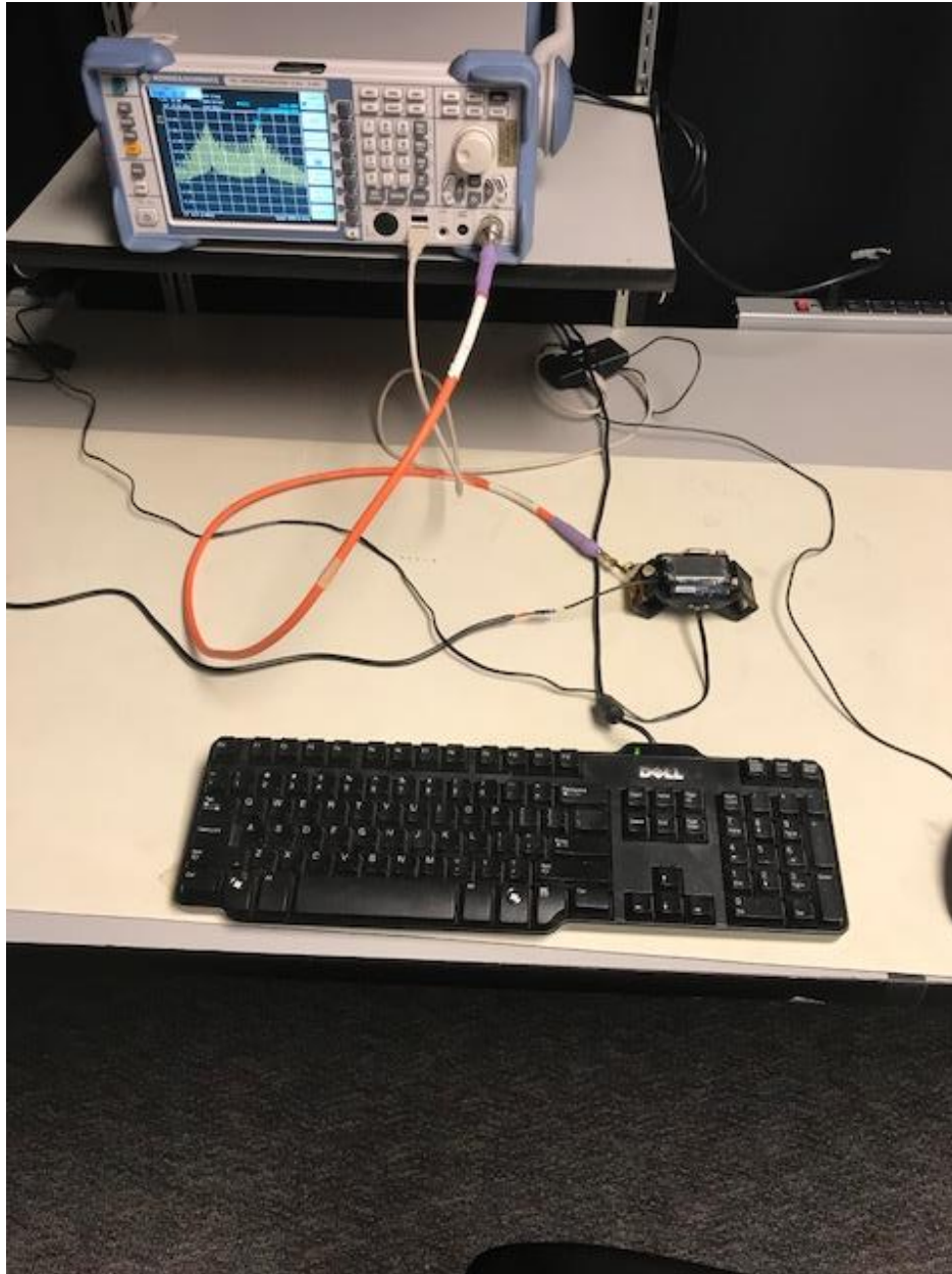
Bench test setup
