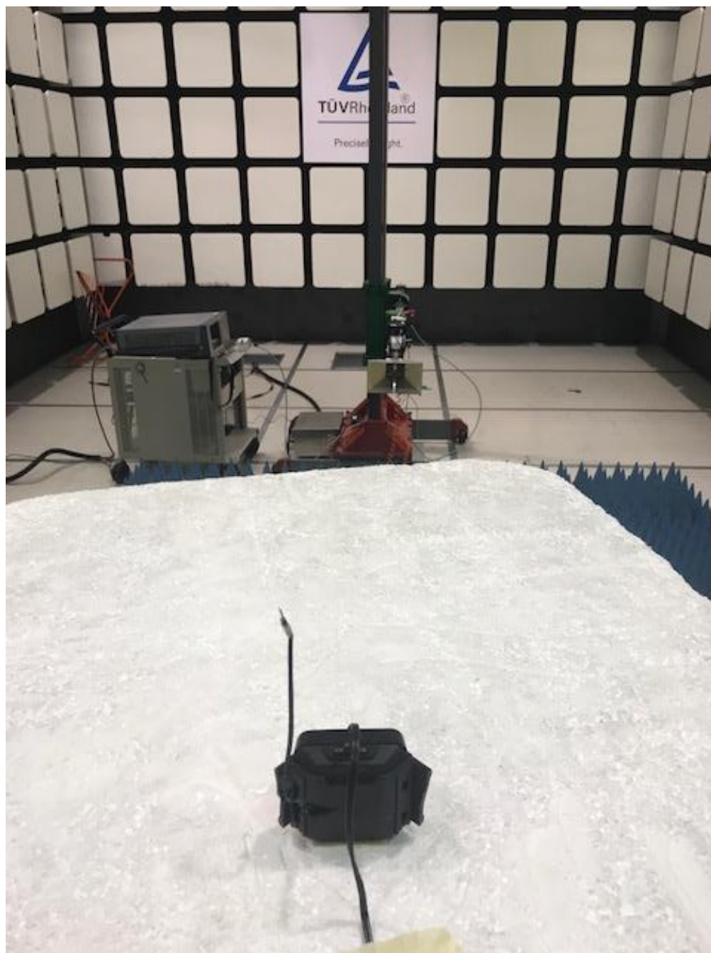
Test Setup 1-18 GHz Rear
