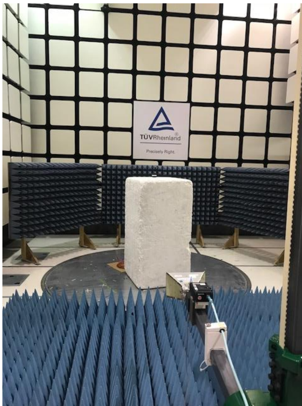
Test Setup 1-18 GHz Front
