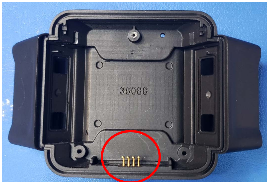
BLUtag V8 Base Enclosure showing Power Connector
