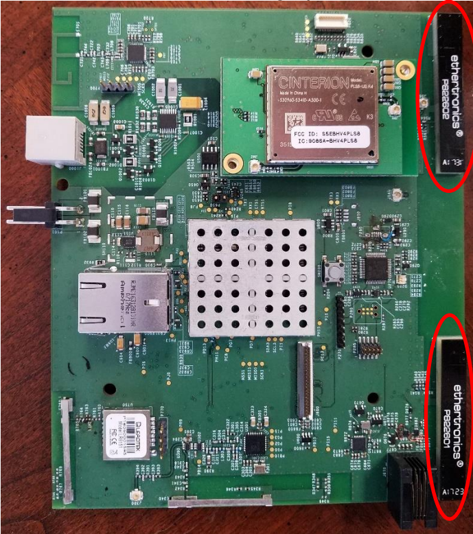
Satellite Tracking of People Modem Module board and Antenna locations. The Antennas are circled.
